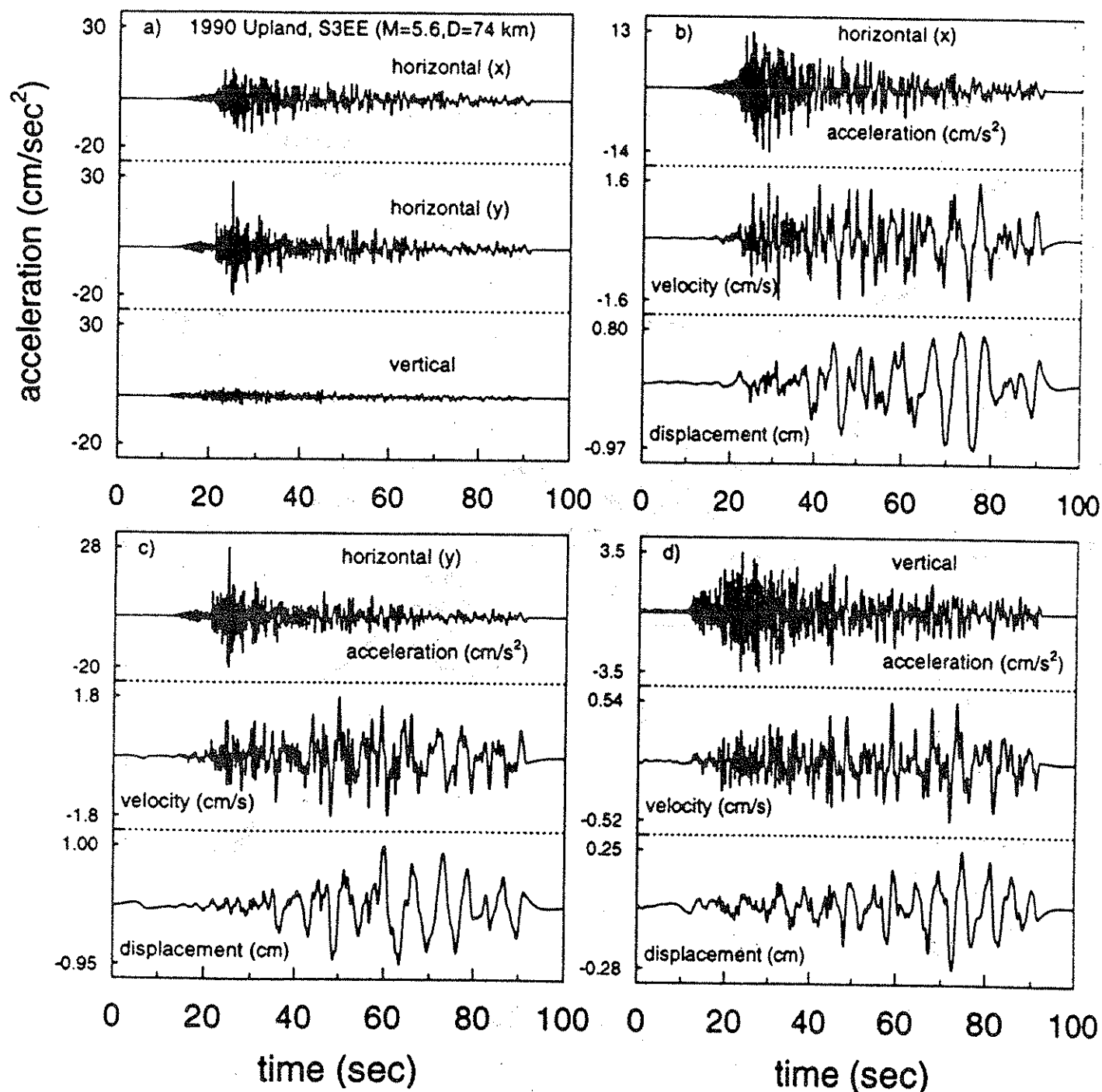
Figure 3. a): Three-component accelerograms, in \text{cm/sec}^2 , of the Upland 1990 earthquake recorded at SEMS station S3EE, plotted using the same vertical scale to emphasize the relative amplitude of the components. The time series are similar to those recorded onshore, with a clear portion of strong S-wave arrivals following the initial P-waves. Two interesting characteristics are the small amplitude of the vertical motion relative to the horizontal motions and the long-period energy arriving after the portion of strongest ground acceleration. b), c), and d): acceleration ( \text{cm/sec}^2 ), velocity ( \text{cm/sec} ), and displacement ( \text{cm} ) time series for the three components of the S3EE recording of the 1990 Upland earthquake, plotted using different vertical scales, to emphasize the appearance of the waveforms. Note the dominance of late arriving 5 to 6 sec waves on the displacement trace, something not emphasized in the accelerogram.
